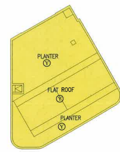
TOP FLOOR PLAN - LEVEL 130.75
